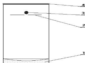
Figure 17: Schematic diagram of Kozyrev's telescope. 1 - focusing mirror, 2 - slit, 3 - detector, 4 - light-tight cover.
