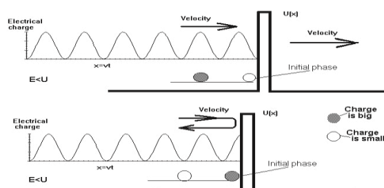
Figure 14: Illustration of the tunnel effect
