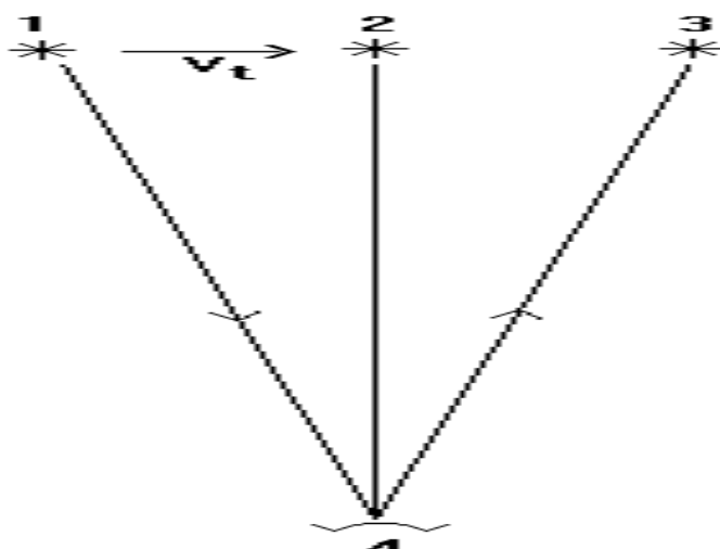
Figure 16: Past (1), present (2), and future (3) positions of an astronomical object. Photons of light emitted by an object at position (1) reach an observer (4) many years later. During this time, the object, moving perpendicular to the observer at velocity V_t , moves to position (2). If, at the moment of fixation, some of the light had been emitted for the observation point, it would have encountered the object at point (3).
