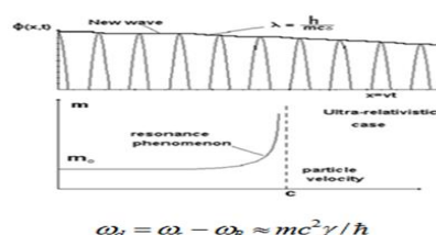
Figure 4: The emergence of a new low-frequency wave.
