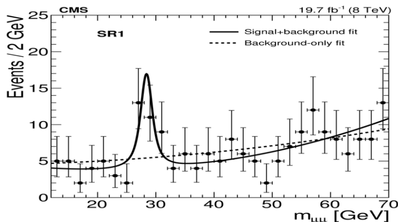
Figure 8: Energy peak at 28 GeV
