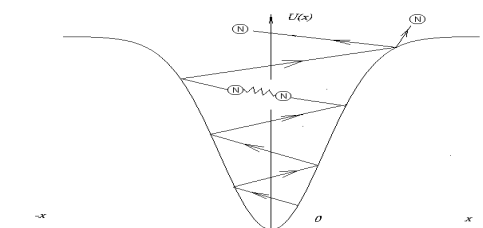
Figure 13: Oscillation of a nitrogen molecule in a catalyst potential well.
