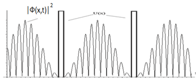
Figure 15: Visual representation of particles passing through two potentials barriers - a diagram of Maxwell's New Demon.
