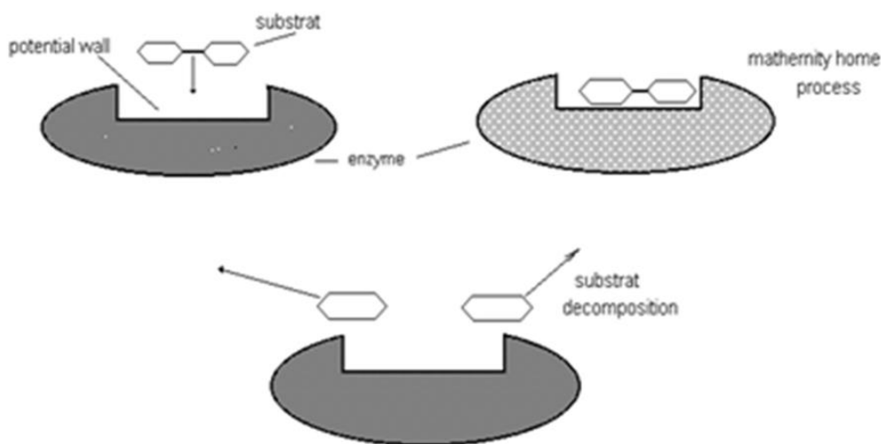
Figure 13: Polysaccharide splitting in the lysozyme molecule. Surprising results have been obtained for the catalytic decomposition
