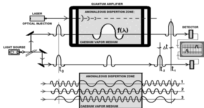
Figure 7: Li Jiu Wang's experiments on superluminal light propagation.
