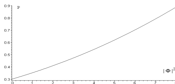
Figure 6: Probability of detecting a P particle in UQT
