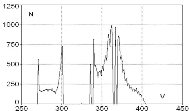
Figure 10: The number of particles passing through 3 barriers with a rectangular distribution of particle velocities from 250 to 450 with arbitrary initial phases
